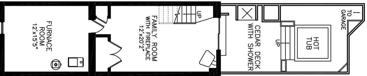
LOWER LEVEL AREA: 540 sq.ft.
